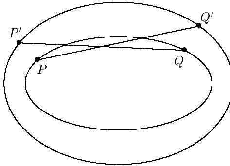
FIGURE 30.7. Ivory's lemma
