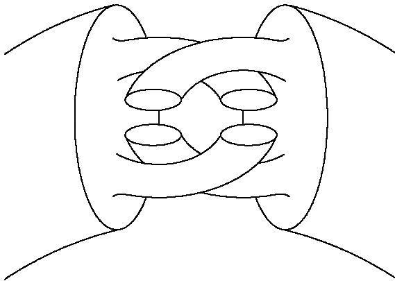
FIGURE 26.5. The lock
