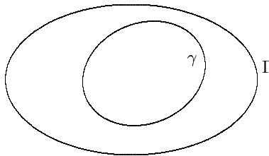
FIGURE 19.4. Nested ovals
