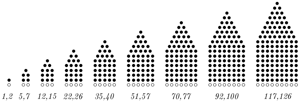
FIGURE 3.1. Pentagonal numbers
