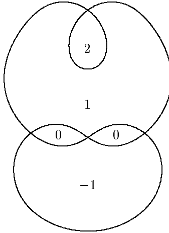
FIGURE 12.20. Rotation numbers
