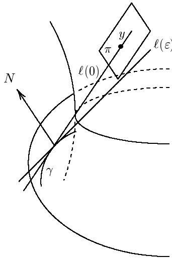
FIGURE 28.15. Proving Theorem 28.9
