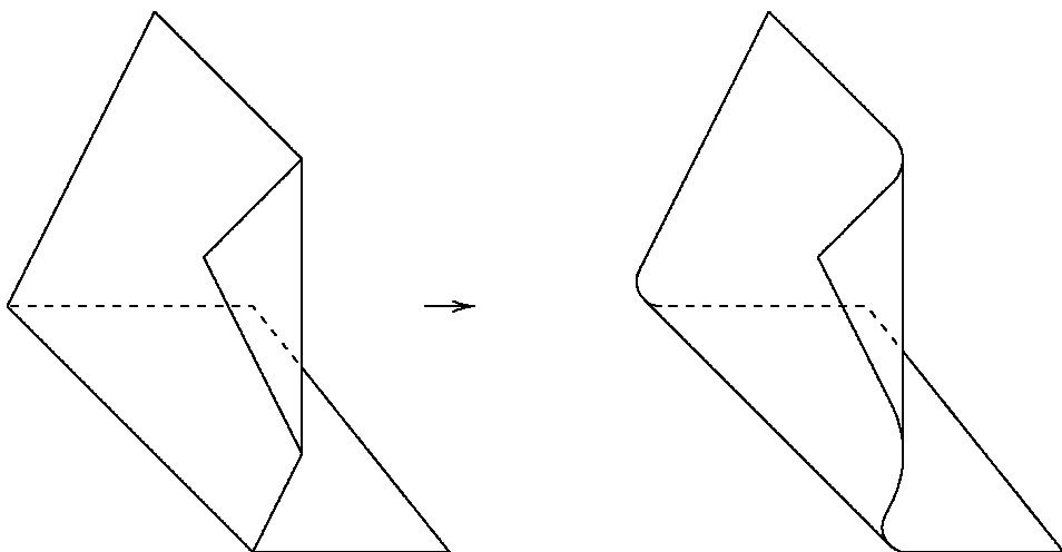
FIGURE 14.8. Rounding folds.
