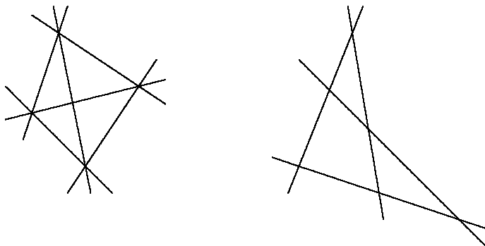
FIGURE 8.6. Dual figures
