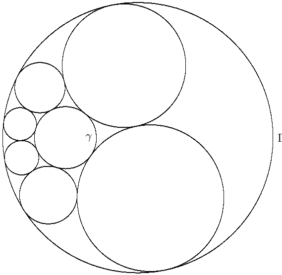
FIGURE 29.6. Steiner's theorem
