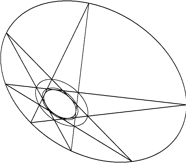
FIGURE 29.5. Poncelet grid
