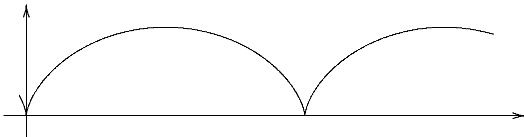
FIGURE 9.2. Cycloid
