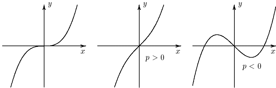
FIGURE 4.1. Cubic parabolas
