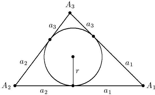
FIGURE 29.10. Proving 6-periodicity
