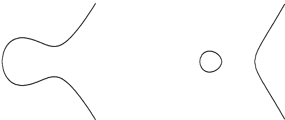
FIGURE 10.16. Cubic curves
