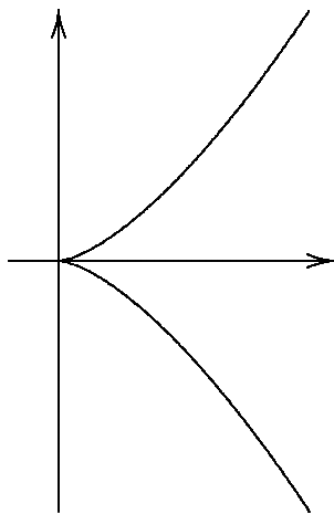
FIGURE 9.1. Semicubic parabola
