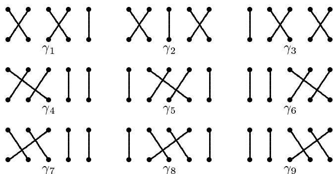
FIGURE 5.8. Permutations \gamma
