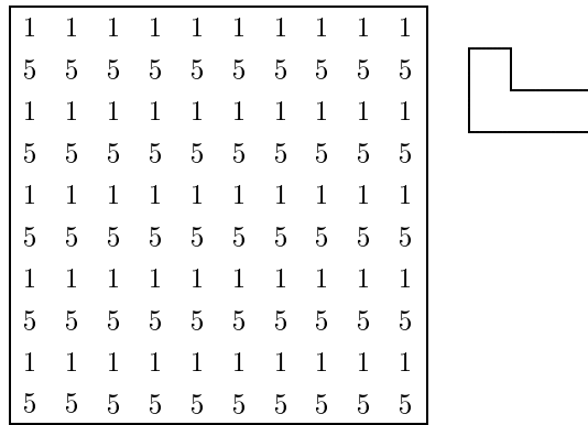
FIGURE 23.4. Coloring modulo 8
