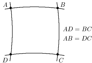
FIGURE 18.16. Chebyshev net
