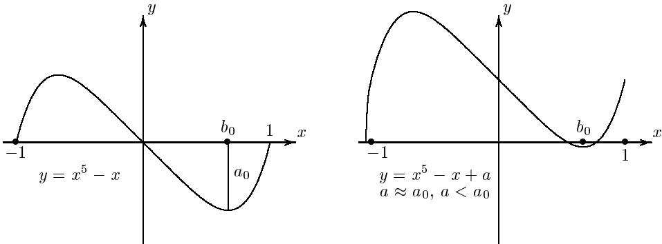
FIGURE 5.10. Two graphs
