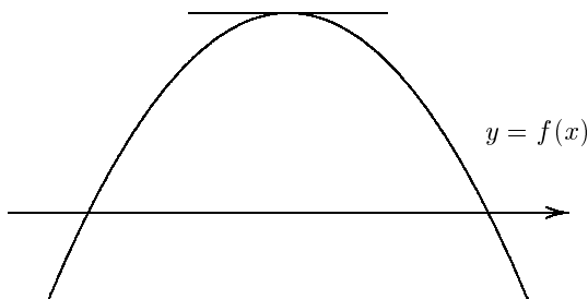
FIGURE 6.1. Rolle's theorem
