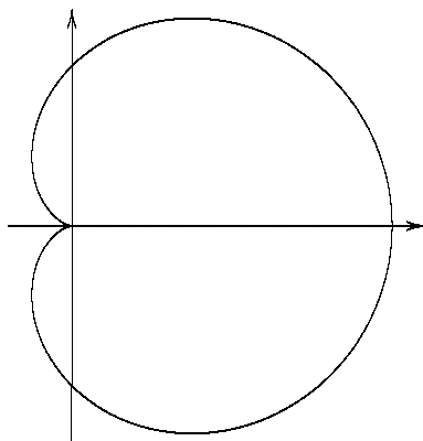
FIGURE 9.3. Cardioid
